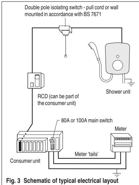
Fig. 3 Schematic of typical electrical layout
