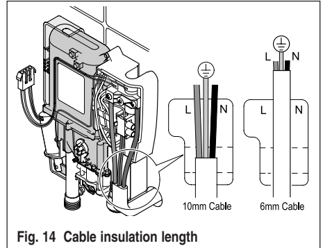
Fig. 14 Cable insulation length
